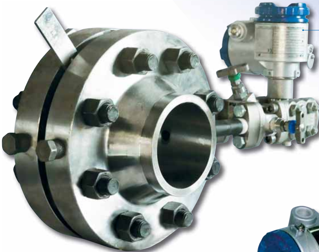
Flow measurement by differential pressure device (orifice plate) for application on gas, liquid and steam.
