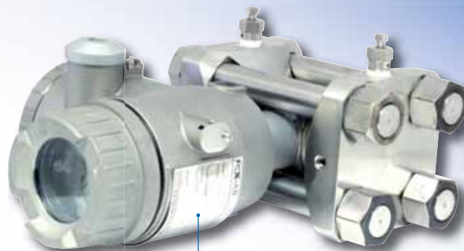
Differential pressure transmitter for high static pressure up to 15 000 Psi (1035 bar).
