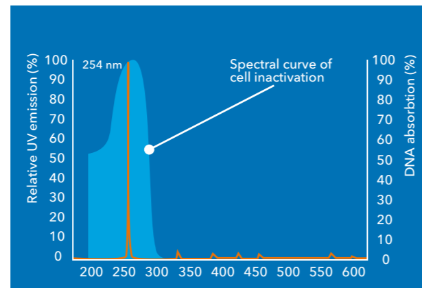
The monochromatic ECORAY UV lamp emits at a wavelength of 254 nm, which is in the maximum of the effective disinfection range of the spectrum
