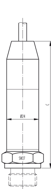
Fig. 3: with process connection
